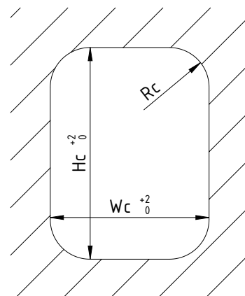
CUT-OUT HOLE IN PLATE (HIP)
